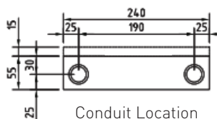
Conduit Location Hinge & Exit Sides
