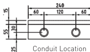
Conduit Location Outlet Sides
