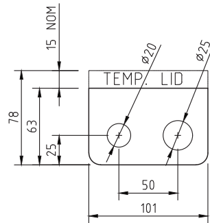
Conduit Location To Sides (Typ.)
